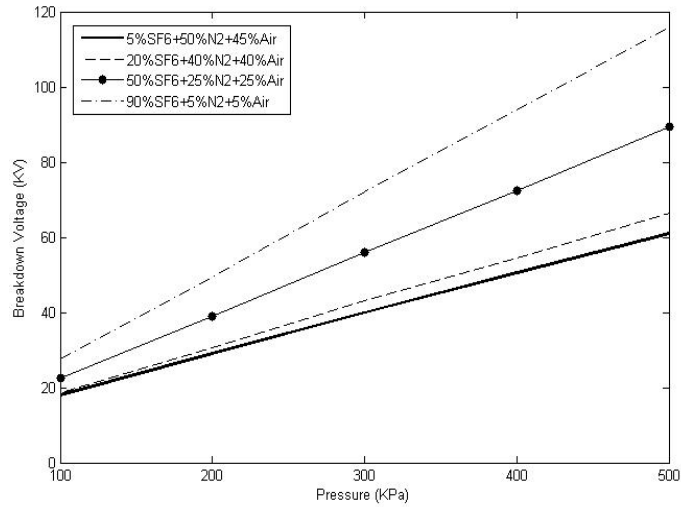
Figure 16. Effect of gas pressure for SF 6 :N 2 :Air mixture on Breakdown Voltage for a gap with particle contamination
