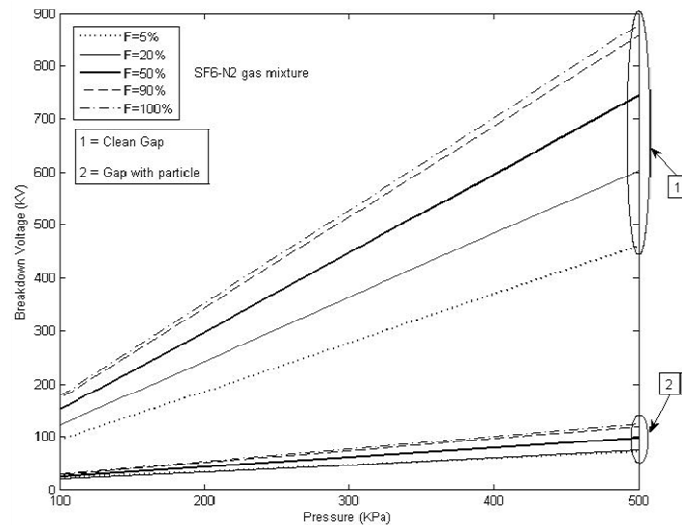
Figure 22. Effect of gas pressure on breakdown voltage for clean gap and gap with particle contamination for a various fractional concentrations of SF 6 -N 2 gas mixture
