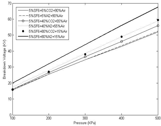
Figure 17. Effect of gas pressure for 5%SF 6 -gas mixture on Breakdown Voltage for a gap with particle contamination
