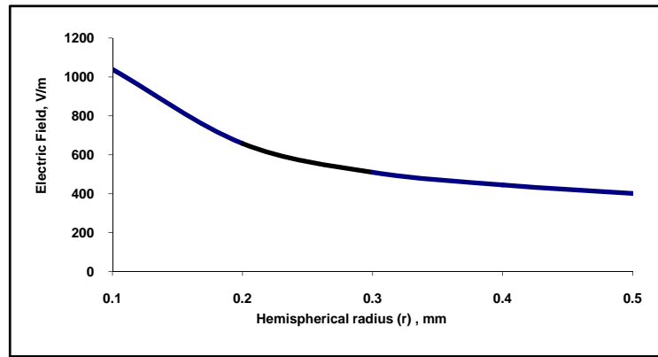
Figure 10. The electric field at upper tip of wire particle versus the particle radius
