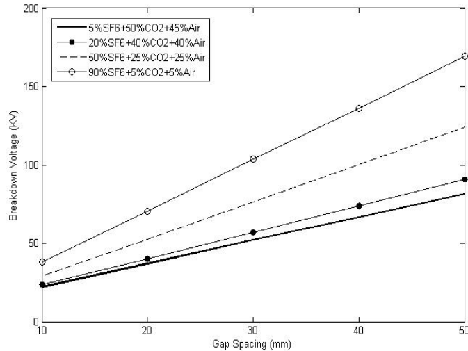
Figure 19. Effect of gap spacing on Breakdown Voltage for SF 6 :CO 2 :Air gas mixture at P=300KPa
