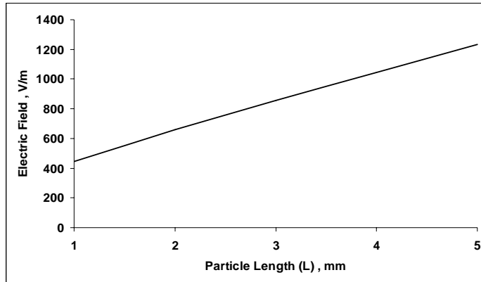
Figure 8. Electric Field at upper tip of wire particle with respect to Particle length
