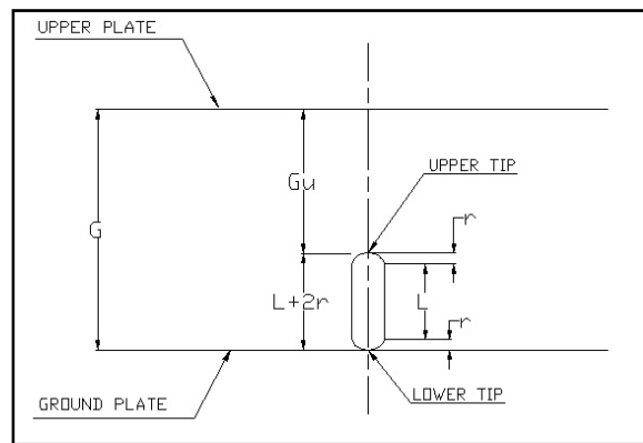
Figure 1. Two parallel plates configuration with filamentary wire contaminating particle resting on earthed electrode
