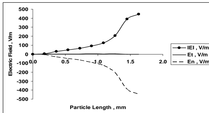
Figure 7. Electric field distribution along surface of wire particle
