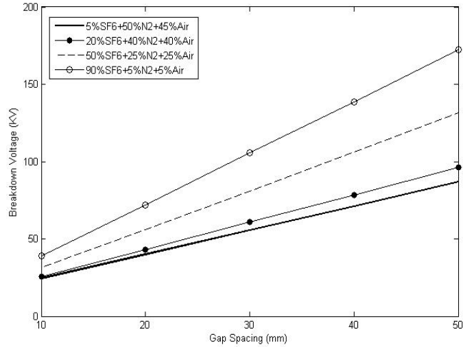
Figure 18. Effect of gap spacing on Breakdown Voltage for SF 6 :N 2 :Air gas mixture at P=300KPa
