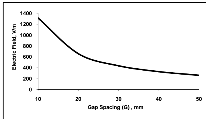
Figure 11. The electric field at upper tip of wire particle versus the gap spacing between two parallel plates
