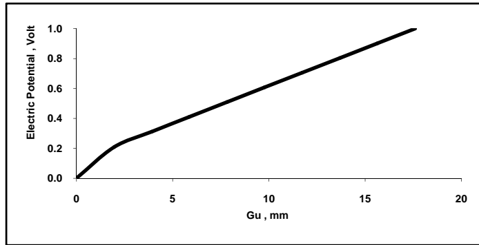
Figure 5. Electric potential distribution along gap from upper tip of wire particle up to upper plate
