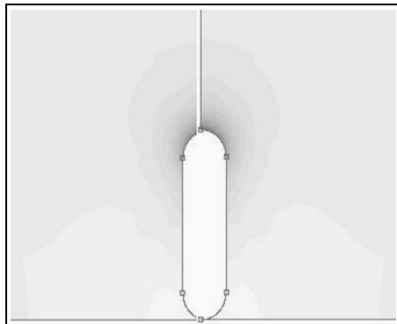
Figure 4. Electric field distribution around wire contaminating particle resting on earthed electrode
