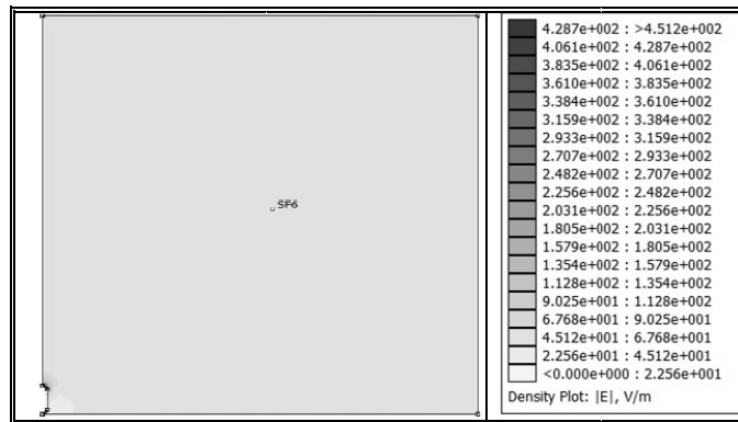
Figure 3. Electric field distribution along gap between two parallel electrodes with wirecontaminating particle resting on earthed electrode
