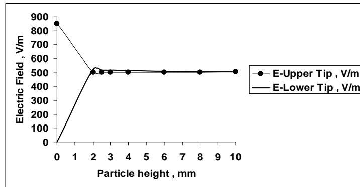
Figure 13. The electric field at the upper tip and the lower tip of the wire particle versus the particle height above the ground plate
