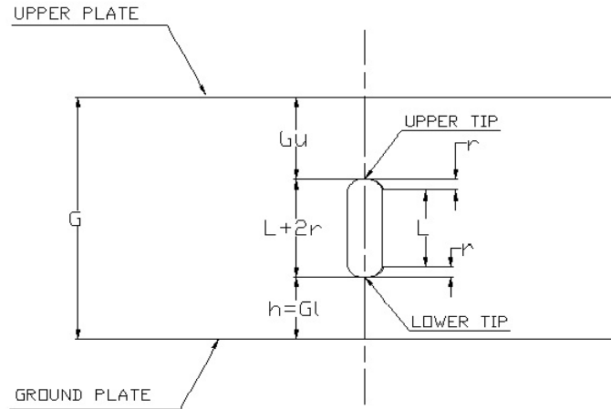
Figure 12. Two parallel electrodes configuration with filamentary wire contaminating Particle hovering in the gap
