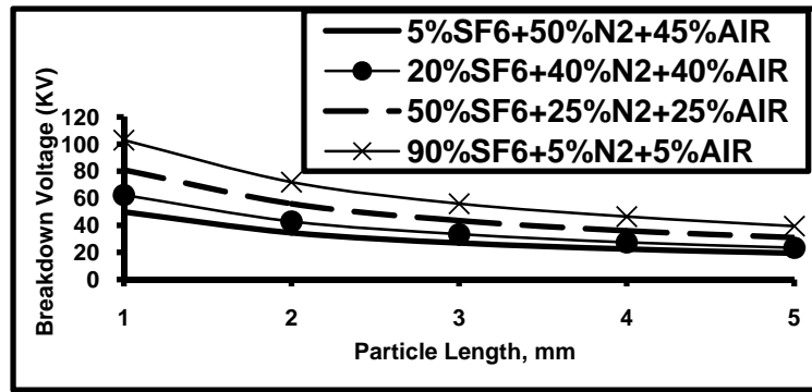
Figure 21. Effect of particle length on Breakdown Voltage for SF 6 :N 2 :Air gas mixture at P=300KPa
