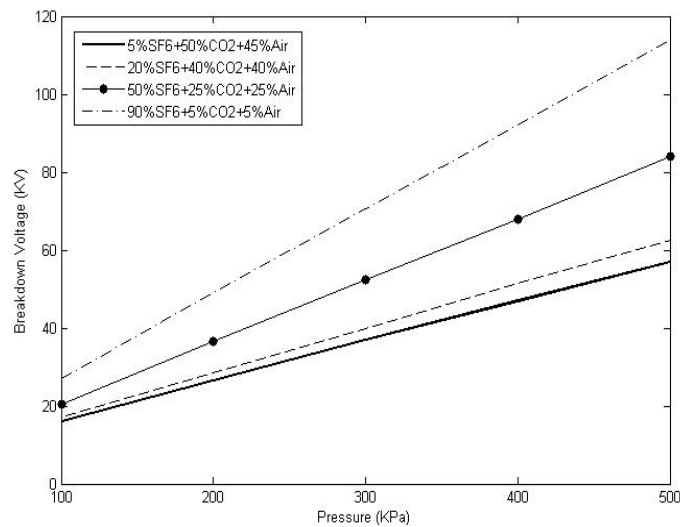
Figure 15. Effect of gas pressure for SF_6:CO_2:Air mixture on Breakdown Voltage for a gap with particle contamination
