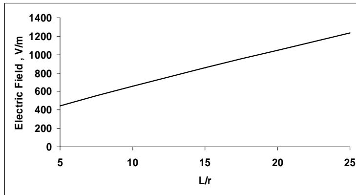
Figure 9. The electric field values at upper tip of wire particle as a function of the ratio (L/r)
