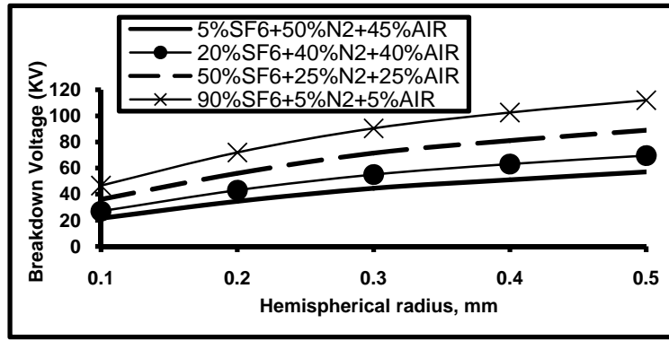
Figure 20. Effect of hemispherical radius of particle on Breakdown Voltage for SF 6 :N 2 :Air gas mixture at P=300KPa
