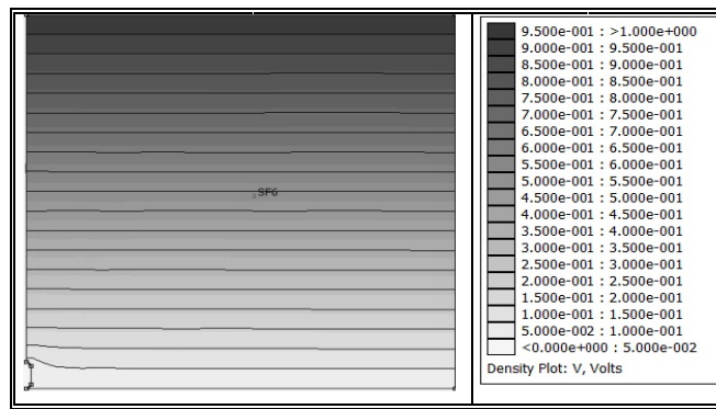
Figure 2. Potential distribution along gap between two parallel plates with wirecontaminating particle resting on earthed electrode
