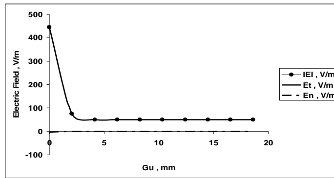
Figure6. Electric field distribution along gap from upper tip of wire particle up to upper plate
